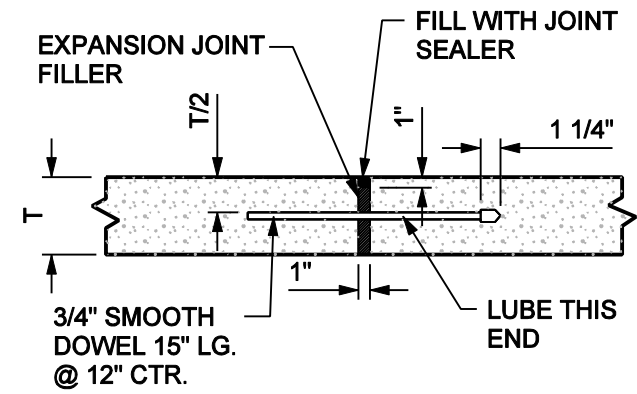
TYPE "A" • ALTERNATE EXPANSION JOINT
