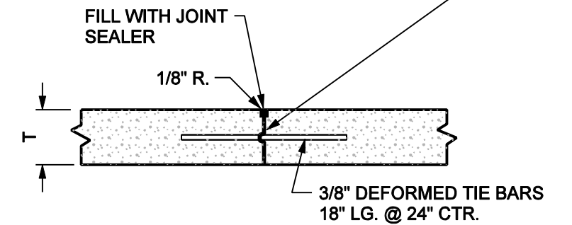
TYPE "E" TIED TRANSVERSE CONSTRUCTION JOINT
