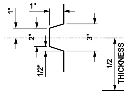
KEY DETAIL
