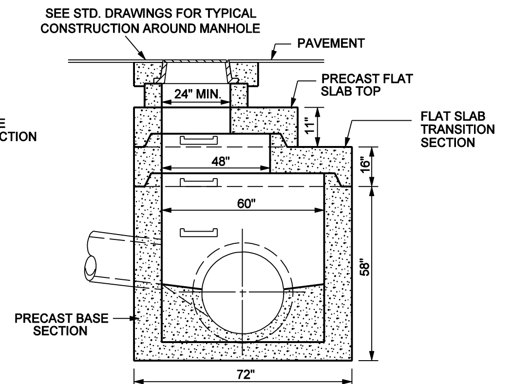
TYPE "E" MANHOLE (FOR SHALLOW SEWERS)
