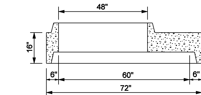
FLAT SLAB TRANSITION SECTION
