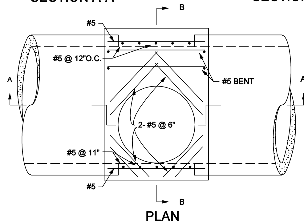
TYPE "C" MANHOLE (FOR SEWERS OVER 48" DIAMETER)
