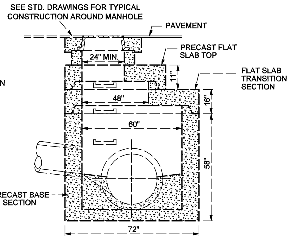
TYPE "E" MANHOLE (FOR SHALLOW SEWERS)
