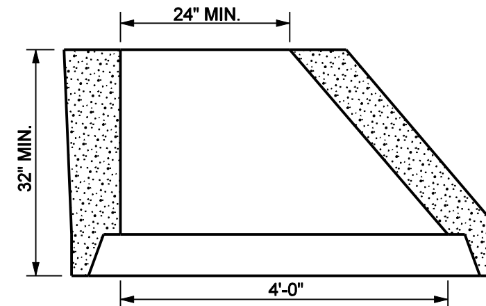
ECCENTRIC CONE
