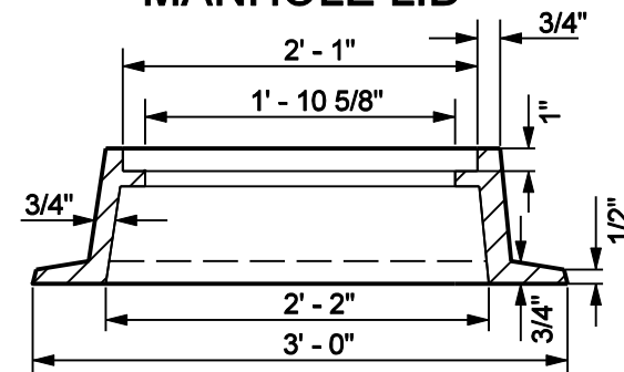
SECTION STORM MANHOLE FRAME AND LID
