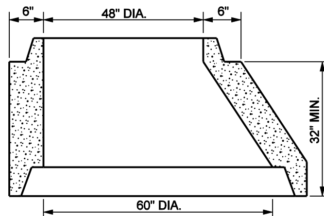
ECCENTRIC REDUCER
