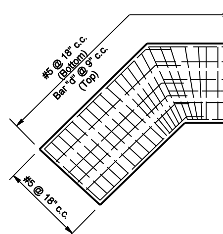
HALF-SECTION B-B
