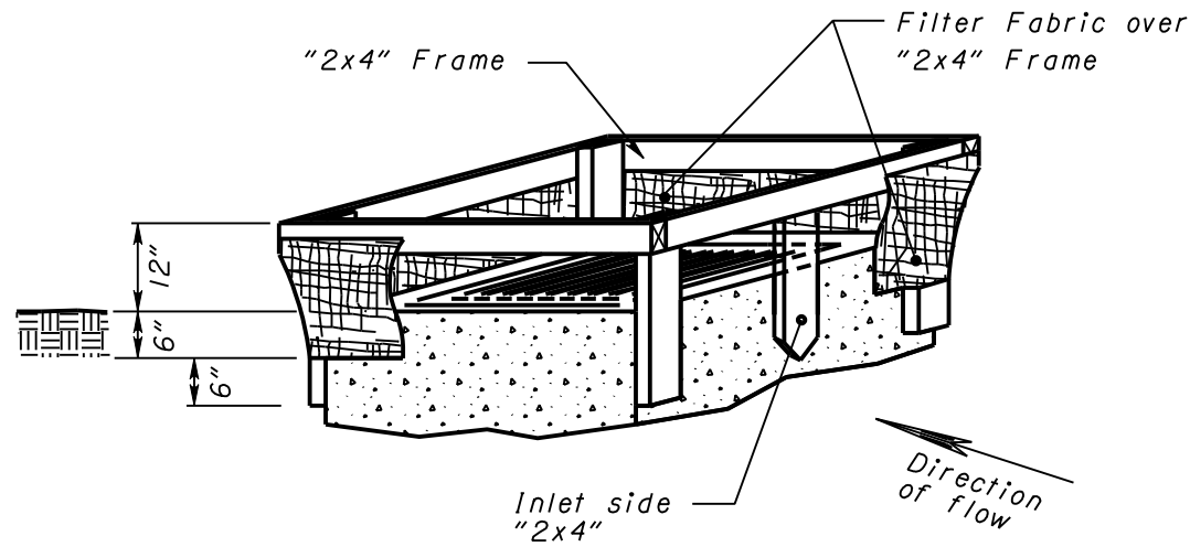
INLET PROTECTION
