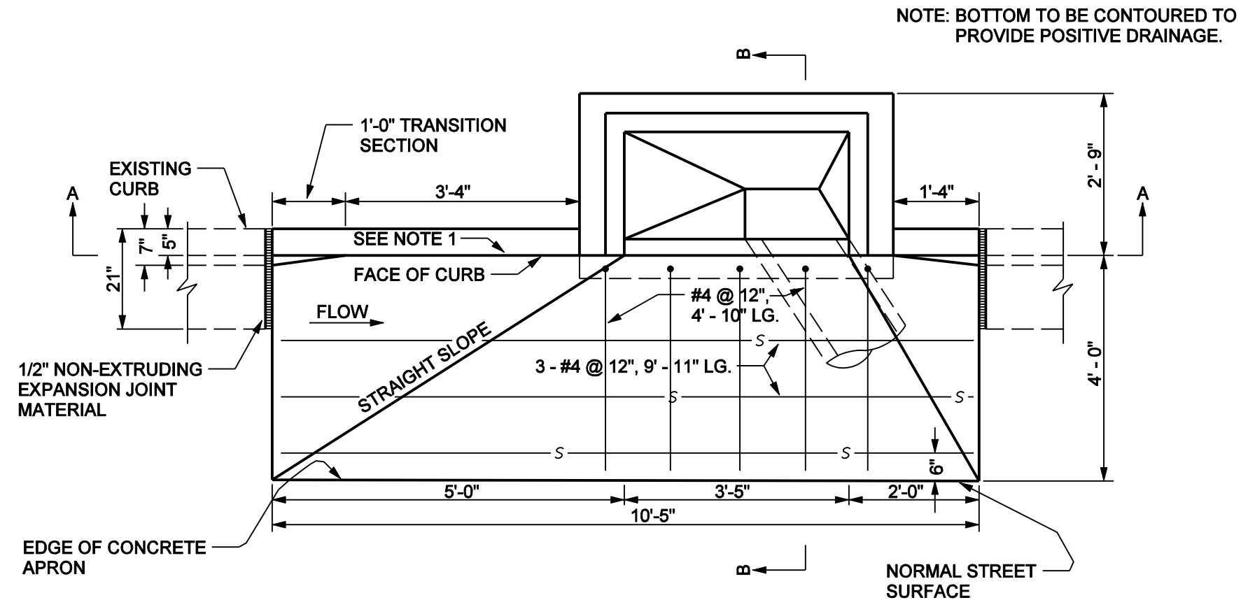
PLAN (WITH COVER REMOVED)
