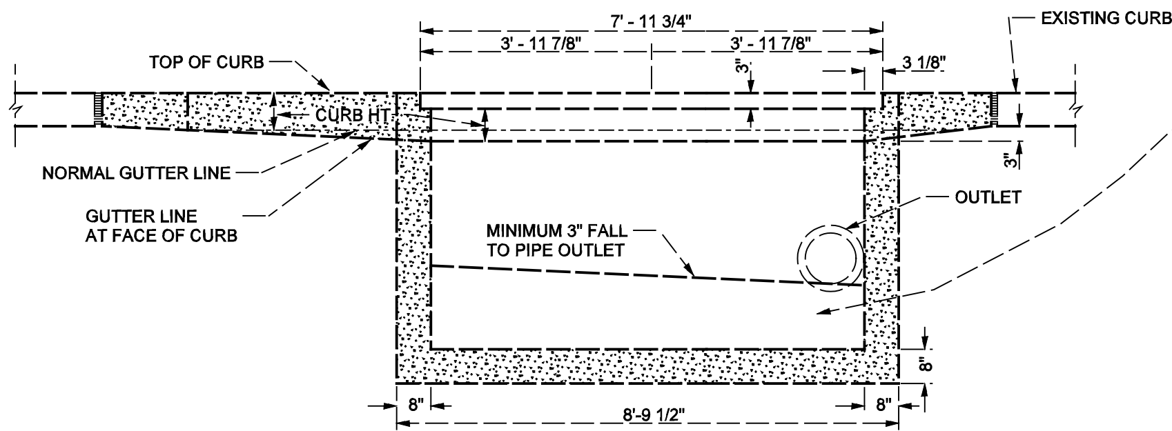
SECTION C - C
