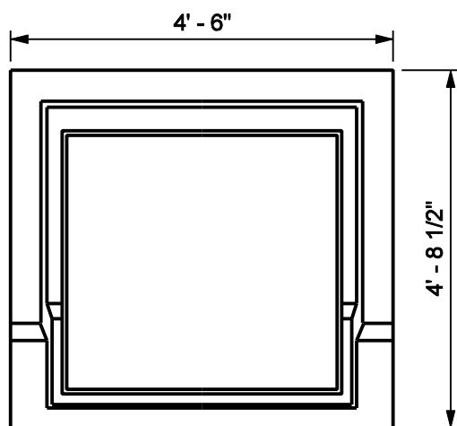
PLAN VIEW WITHOUT COVER OR GRATING
