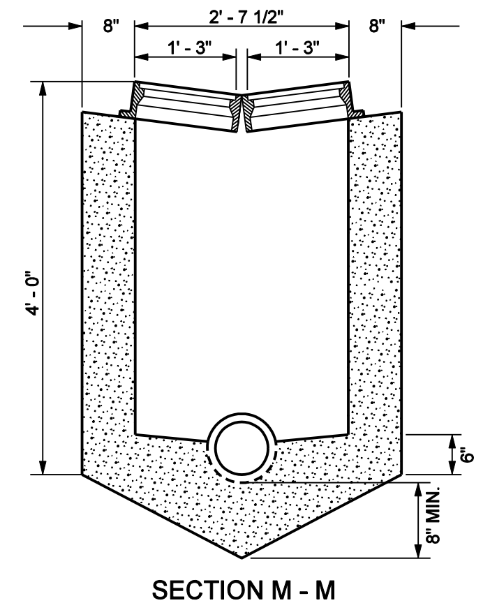
TYPE "E" CATCH BASIN
