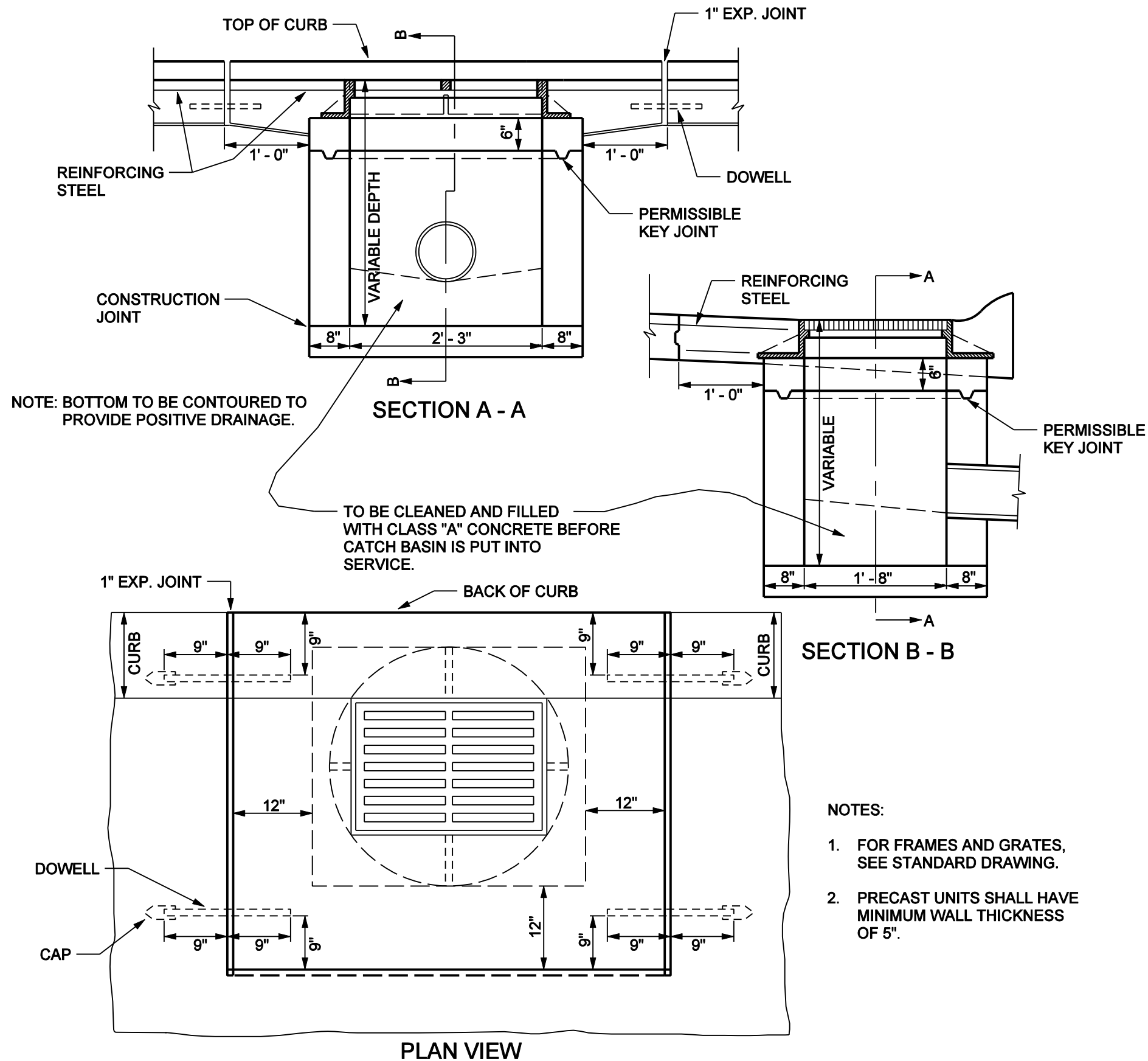
TYPE "F" CATCH BASIN
