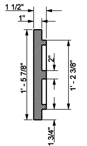
SECTION F - F
