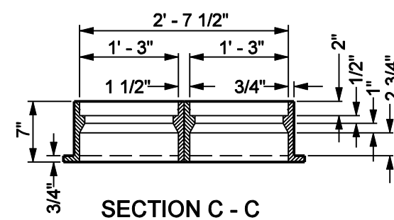
FRAME FOR TYPE "E" CATCH BASIN
