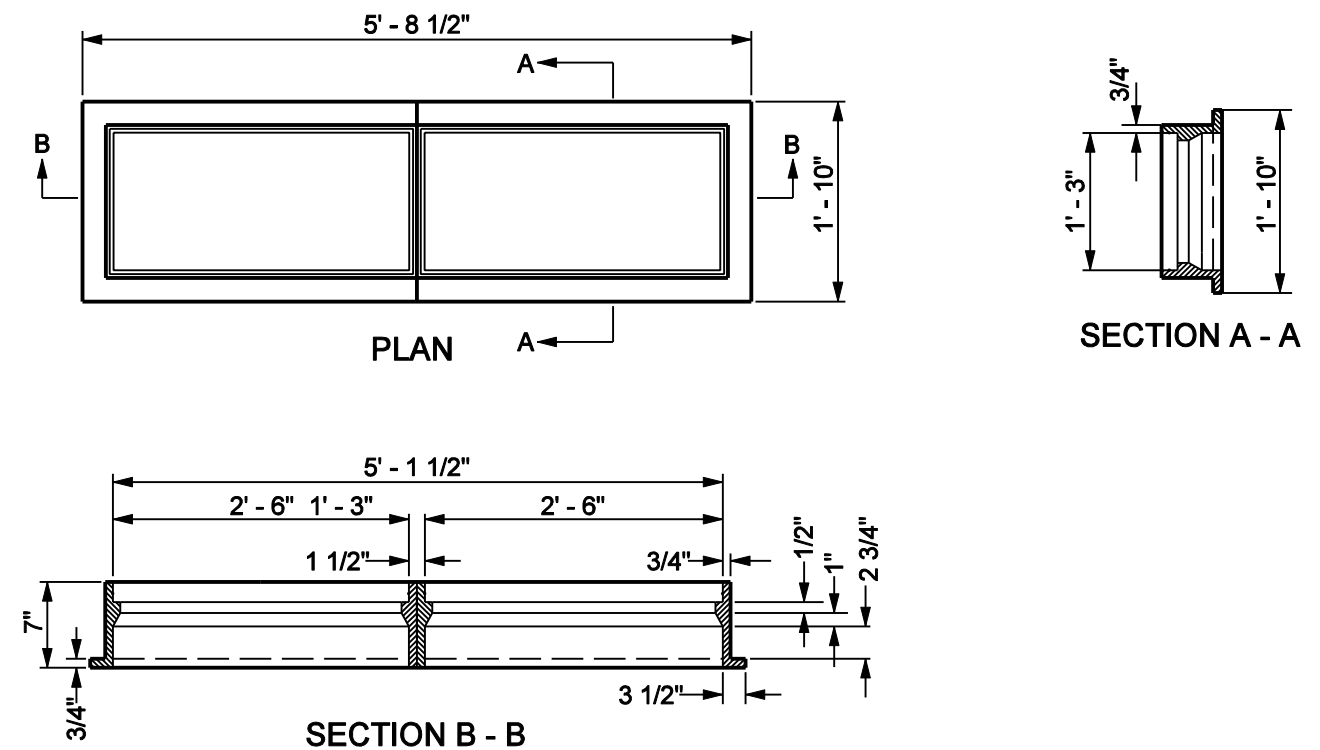
FRAME FOR TYPE "C" CATCH BASIN
