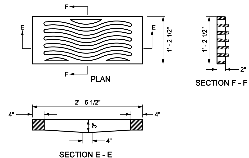
LID FOR TYPE "C" AND "E" CATCH BASINS
