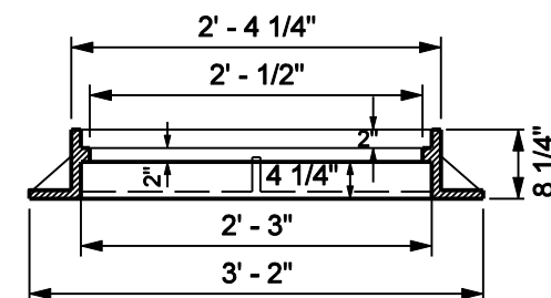
SECTION D - D
