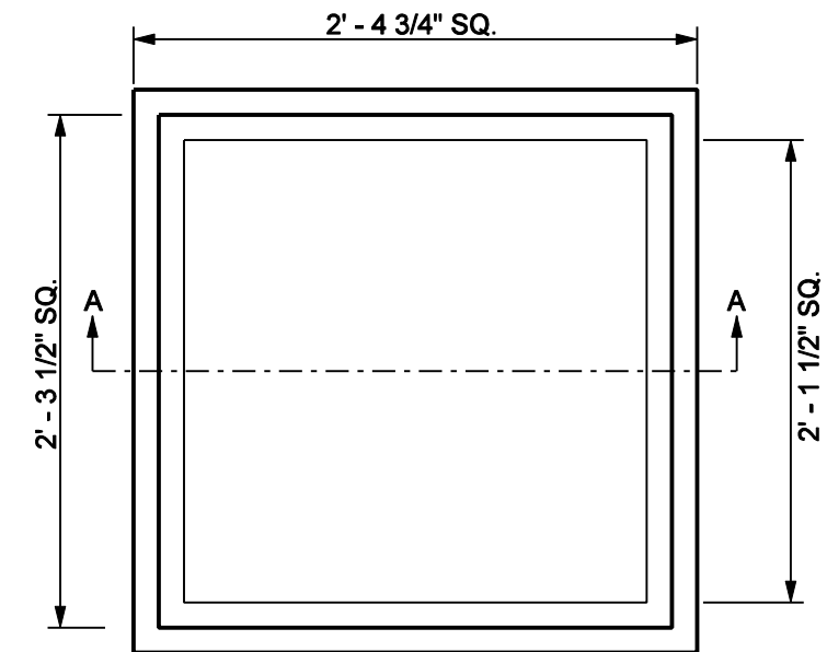
PLAN - FRAME
