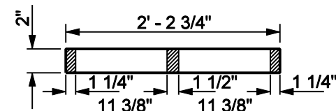
SECTION X - X
