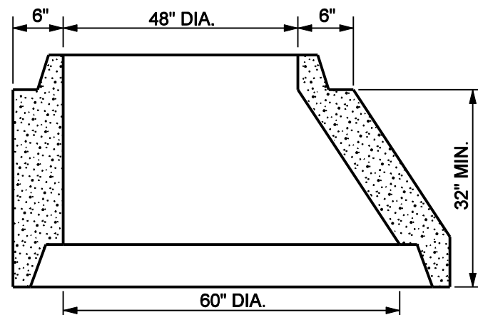
ECCENTRIC REDUCER
