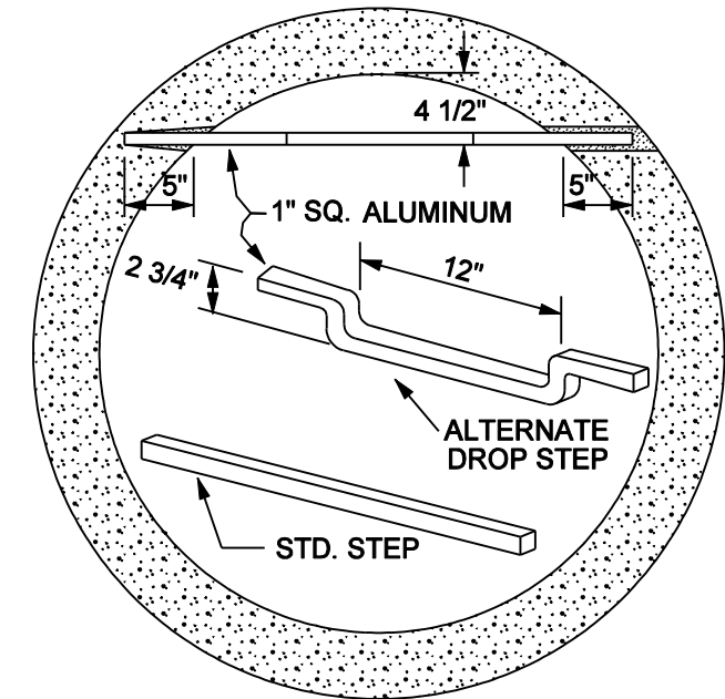
STANDARD SECTION THRU MANHOLE
