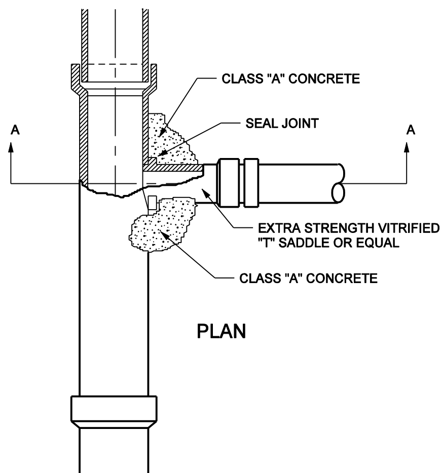
SADDLE DETAIL
