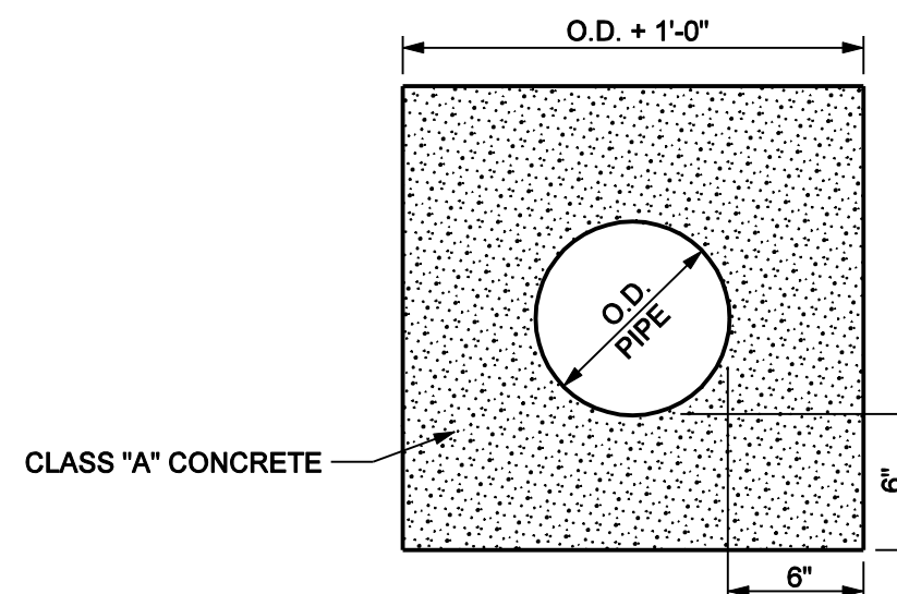
CONCRETE ENCASEMENT DETAIL
